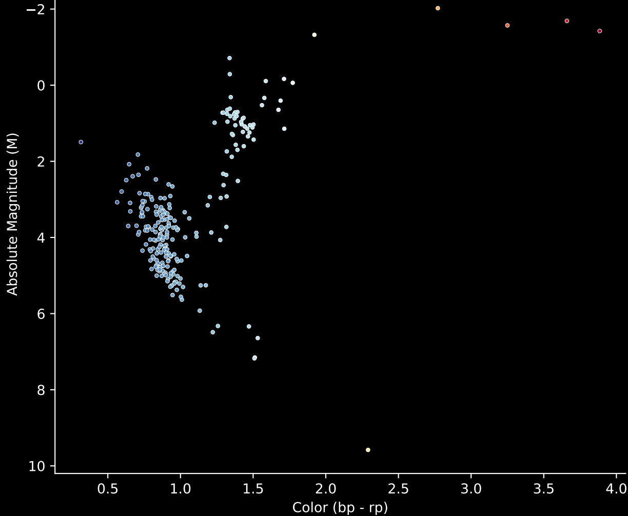
GALAH DR4 Field [7169] Stars (n= 246) Hertzsprung-Russel Diagram
