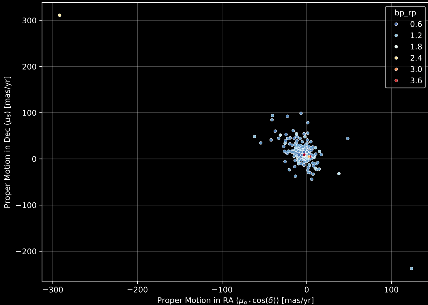
GALAH DR4 Field: [7169] Proper Motion Diagram (n= 246)
