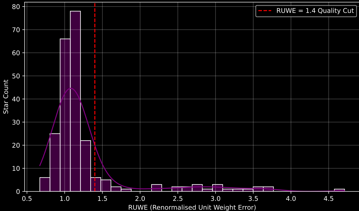
GALAH DR4 Field [7169] RUWE Distribution (n= 233)
