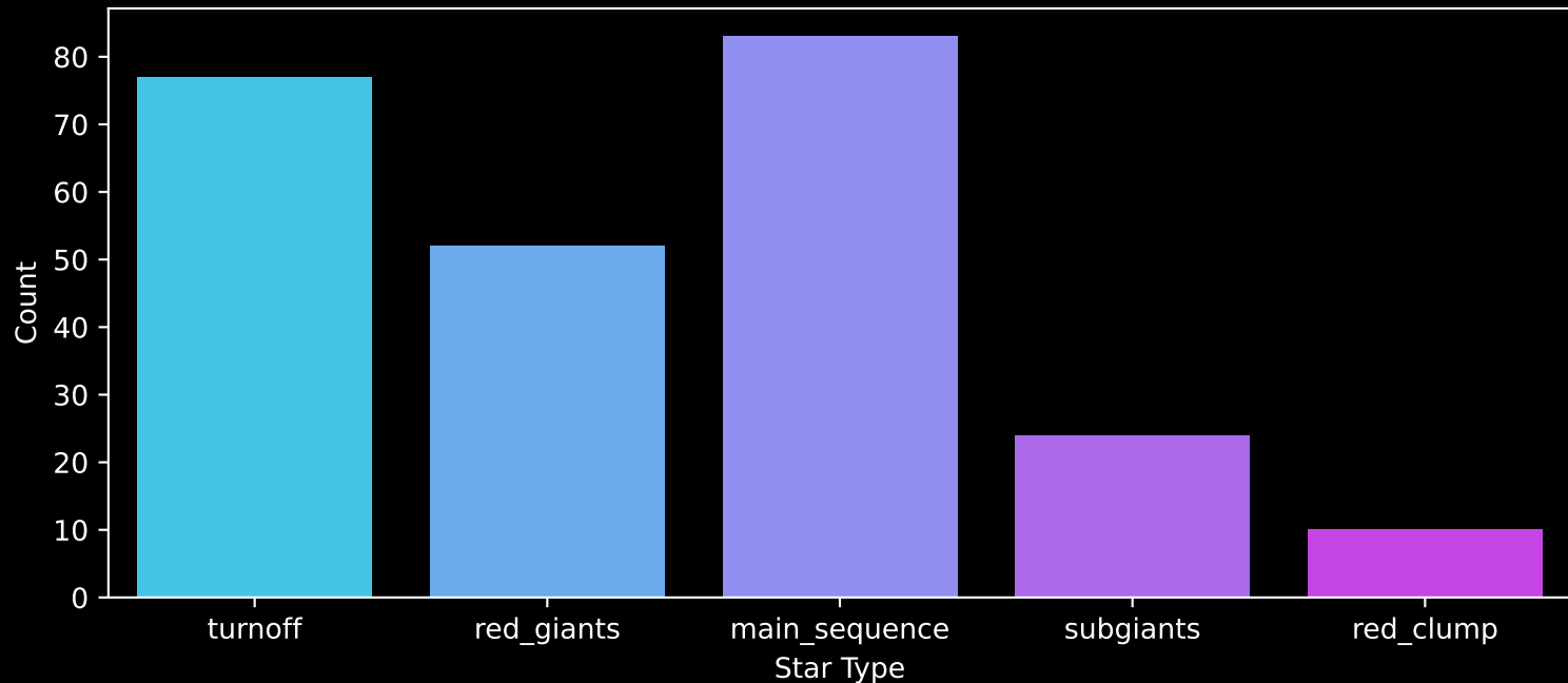
GALAH DR4 Field: [7169] Count plot of Star Type
